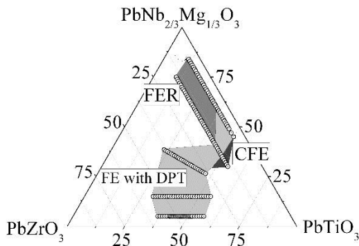
Figure 1. The phase diagram of the system \text{PbZrO}_3\text{-PbNb}_{2/3}\text{Mg}_{1/3}\text{O}_3\text{-PbGeO}_3 , highlighted areas refers to different FE properties of solid solutions.
