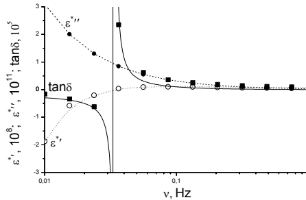
Figure 1. Experimental dielectric spectra of 0.6BiFeO 3 -0.4CdTiO 3 ceramics at 923 K (points) and calculated frequency dependences of ε*, ε*'' and tan δ.
