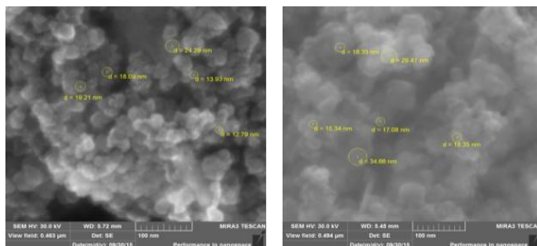
Figure 1. Image of ferrite made with the help of electronic microscopy ( \text{NiFe}_2\text{O}_4 ) on REM (coprecipitation, stabilizer \text{C}_{17}\text{H}_{33}\text{COOH} , T = 80^\circ\text{C} ).
